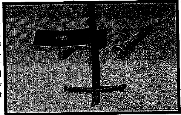
Deck Clip installed in Cumaru decking. Note how the clip bows down holding both sides of the decking tight like a miniature spring.
